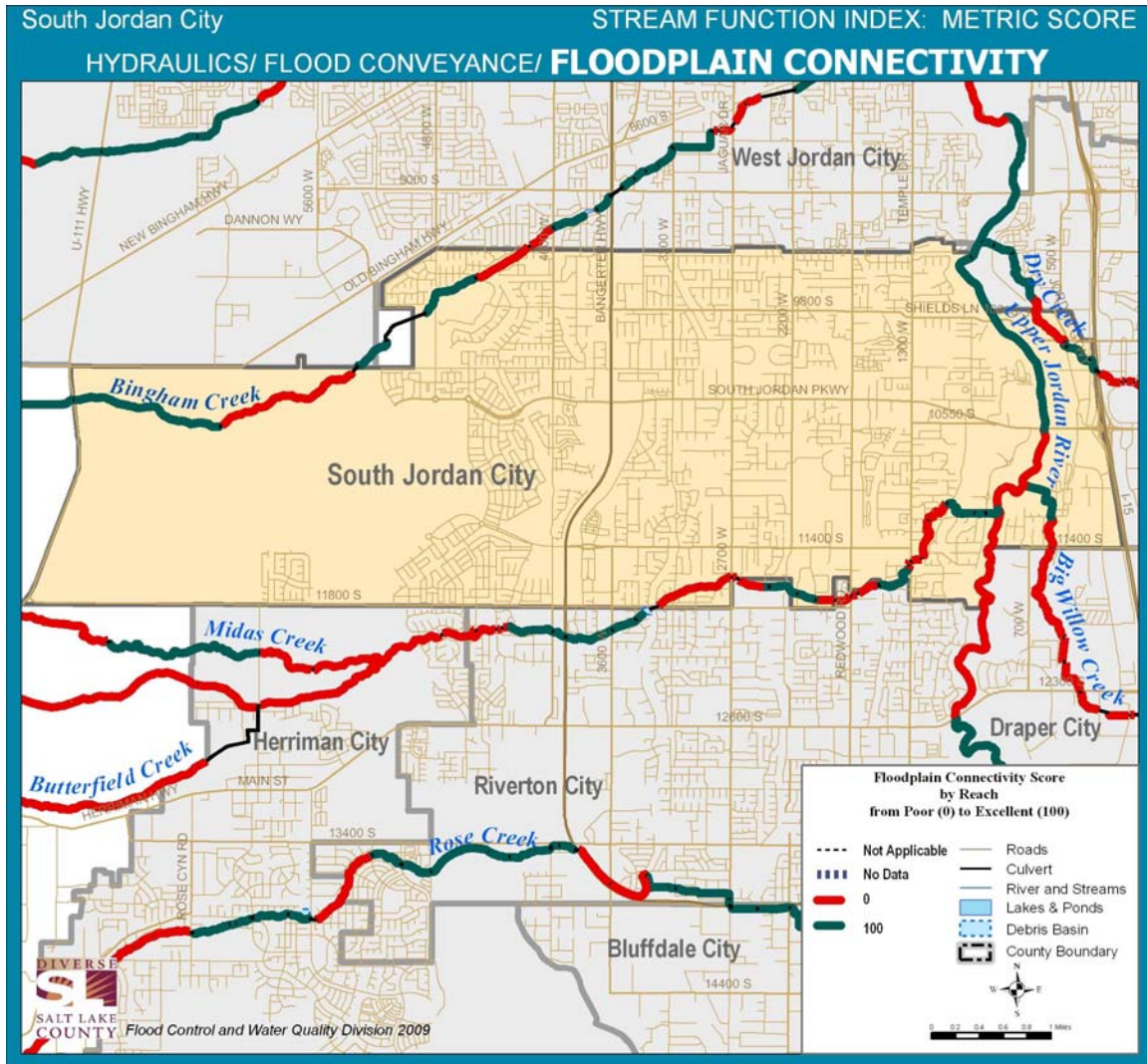
Figure 12. Hydraulics Function—Floodplain Connectivity in South Jordan City
