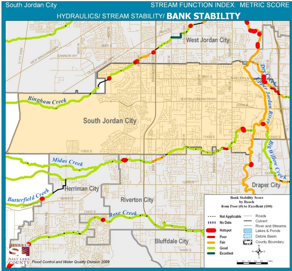
Figure 14. Hydraulics Function—Bank Stability in South Jordan City
